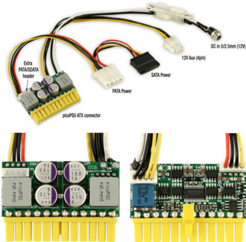
picoPSU-160-XT DC/DC (160 Watt) + AC/DC 120W Adapter + power cord [Bundle]
